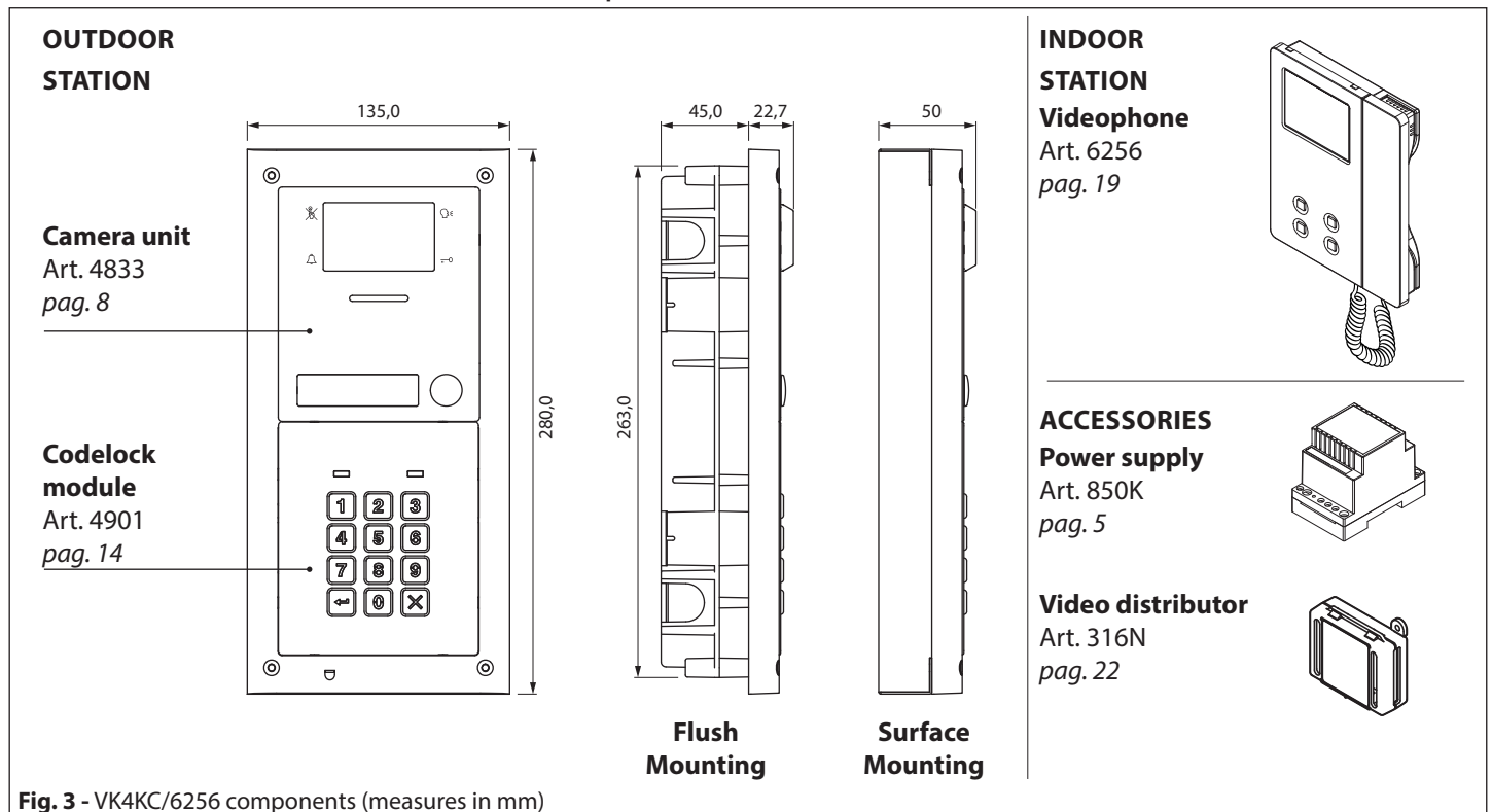
Fig. 3 - VK4KC/6256 components (measures in mm)
